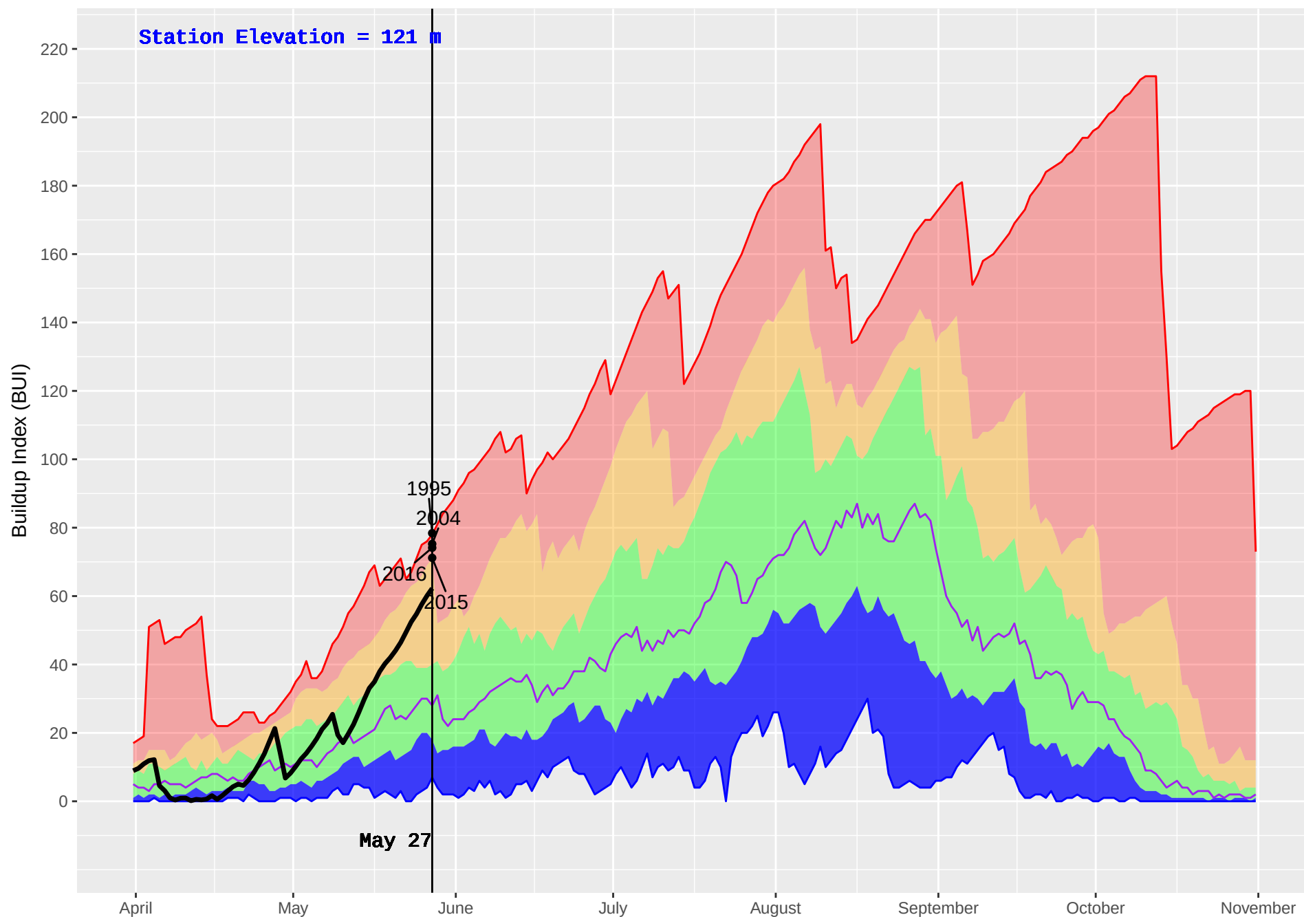
BOWSER (56) : Historical (1985–2016) and Current (2018) Noon Buildup Index (BUI)
