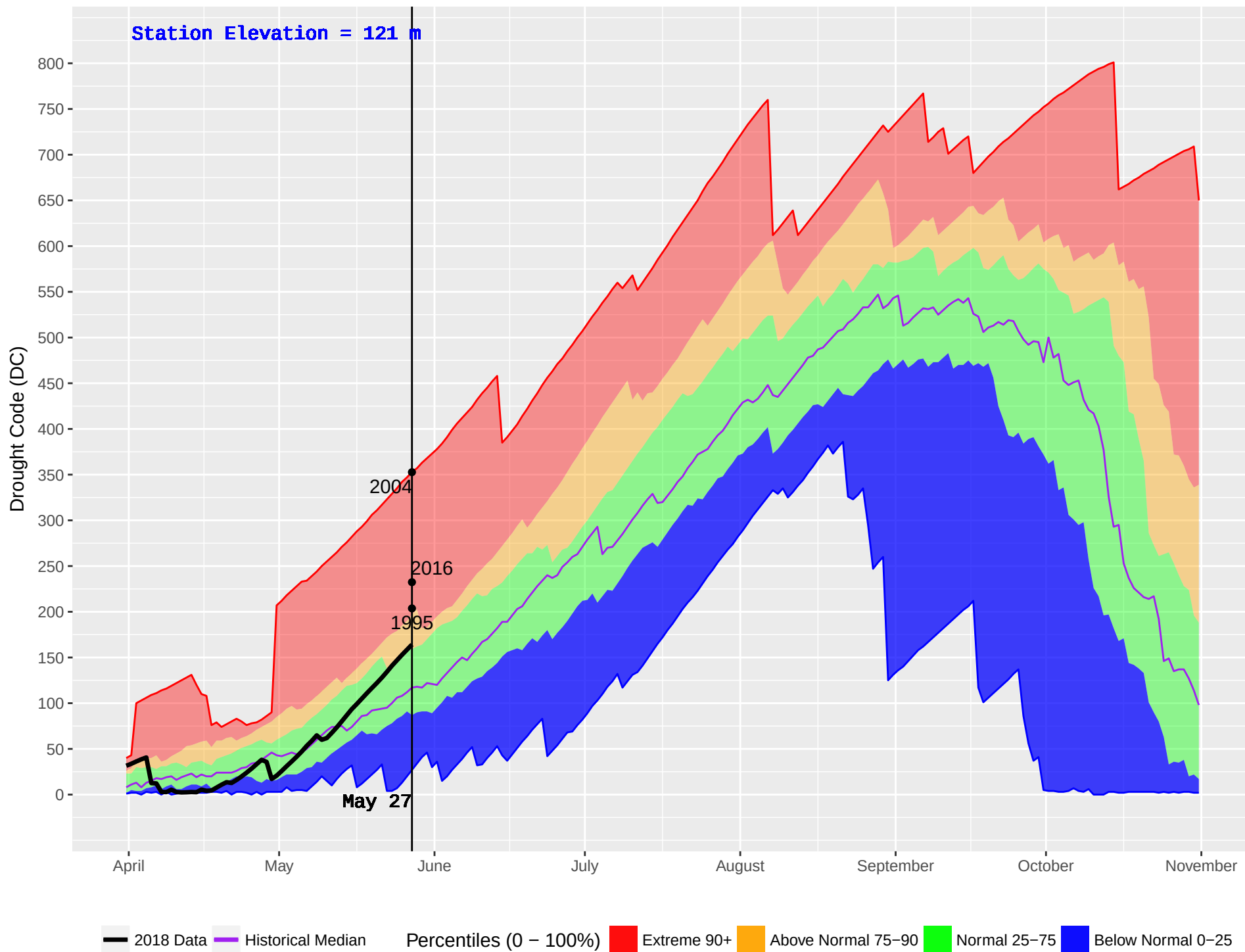
BOWSER (56) : Historical (1985–2016) and Current (2018) Noon Drought Code (DC)
