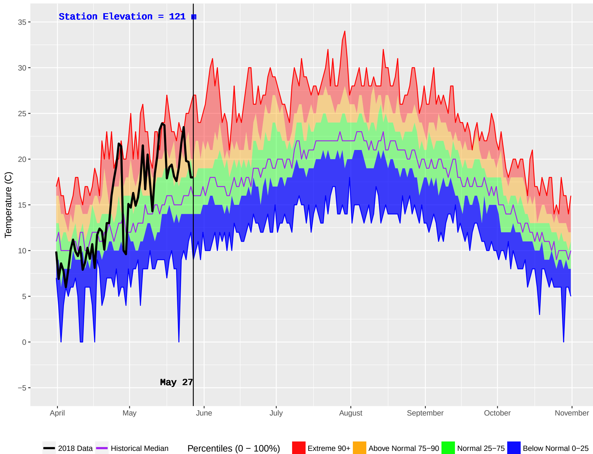
BOWSER (56) : Historical (1985–2016) and Current (2018) Noon Temperature
