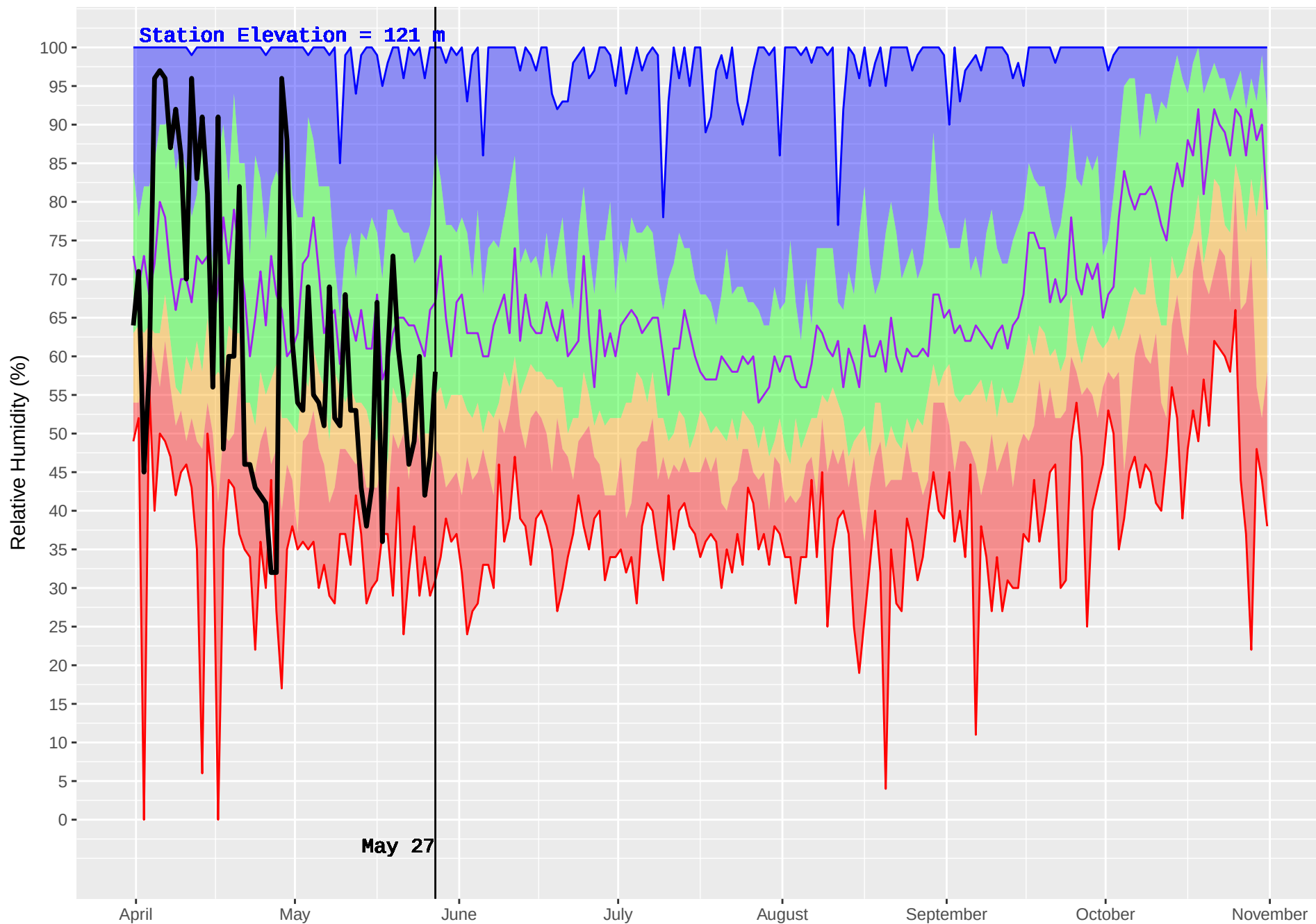
BOWSER (56) : Historical (1985–2016) and Current (2018) Noon Relative Humidity
