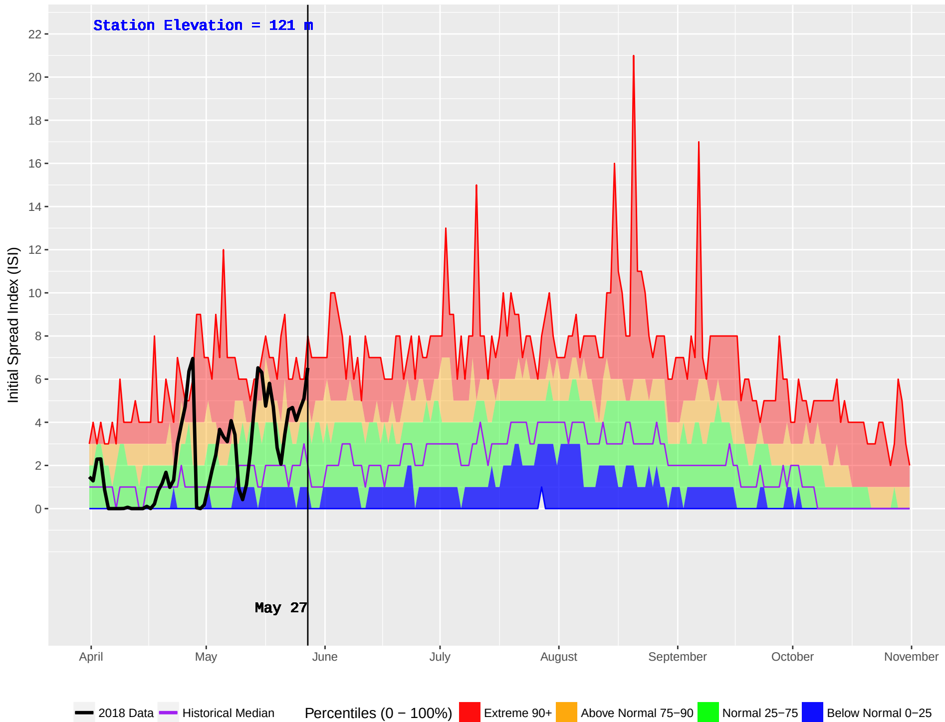
BOWSER (56) : Historical (1985–2016) and Current (2018) Noon Initial Spread Index (ISI)
