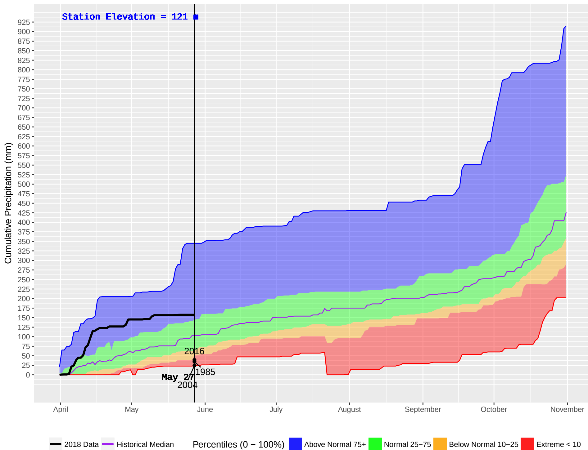
BOWSER (56) : Historical (1985–2016) and Current (2018) Noon Cumulative Precipitation
