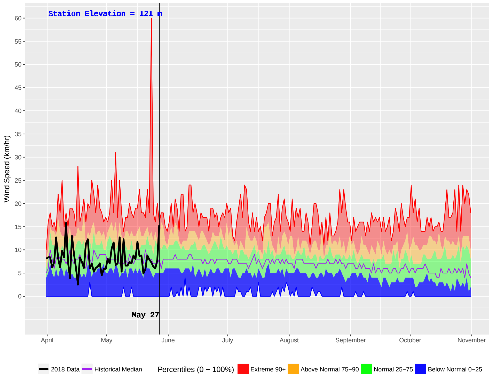
BOWSER (56) : Historical (1985–2016) and Current (2018) Noon Wind Speed
