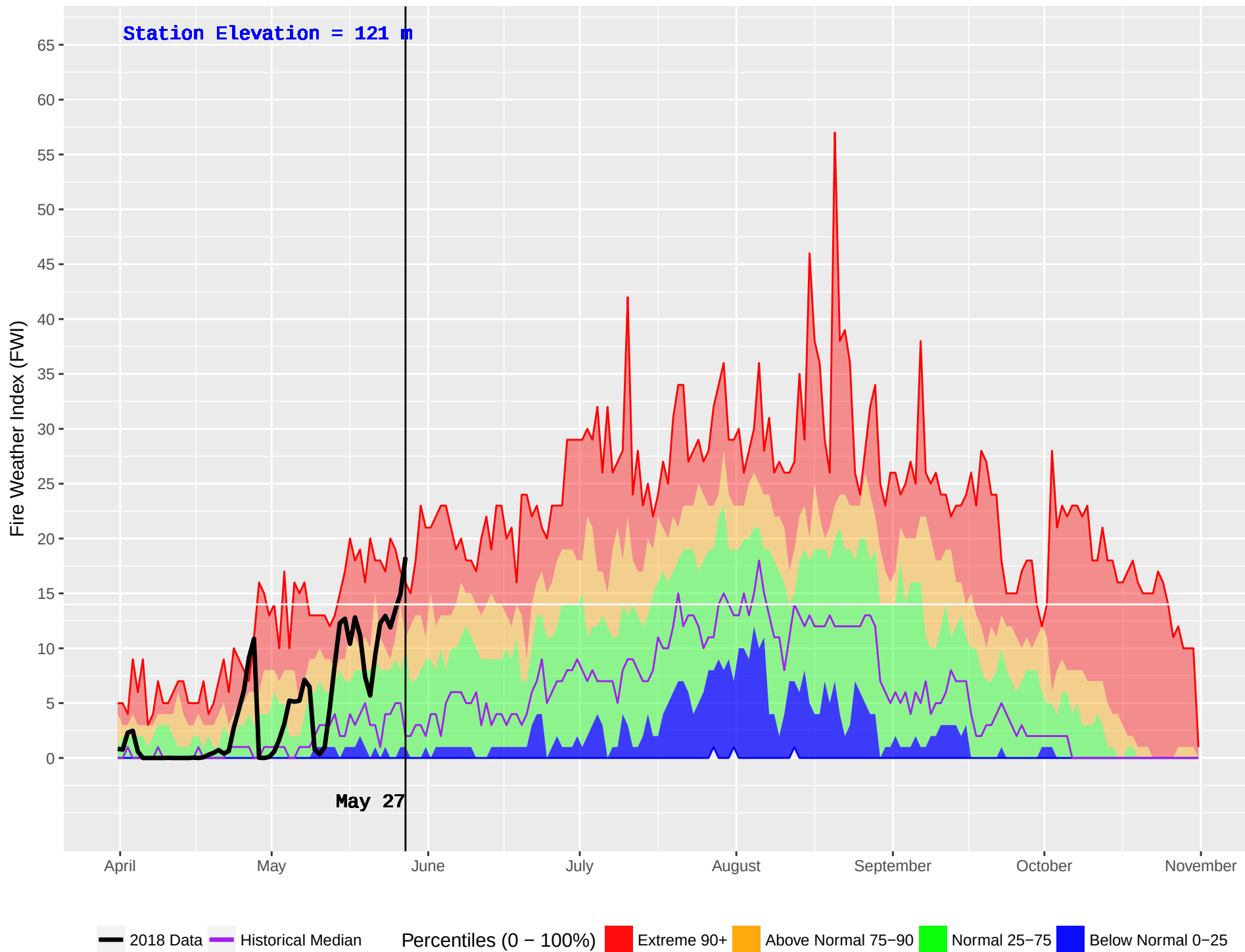
BOWSER (56) : Historical (1985–2016) and Current (2018) Noon Fire Weather Index (FWI)
